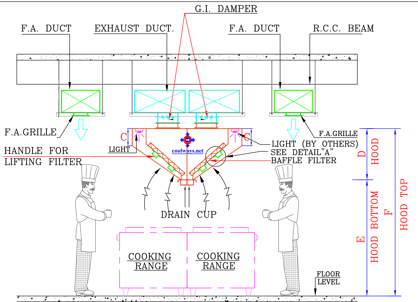
ISLAND TYPE CEILING SUSPENDED
