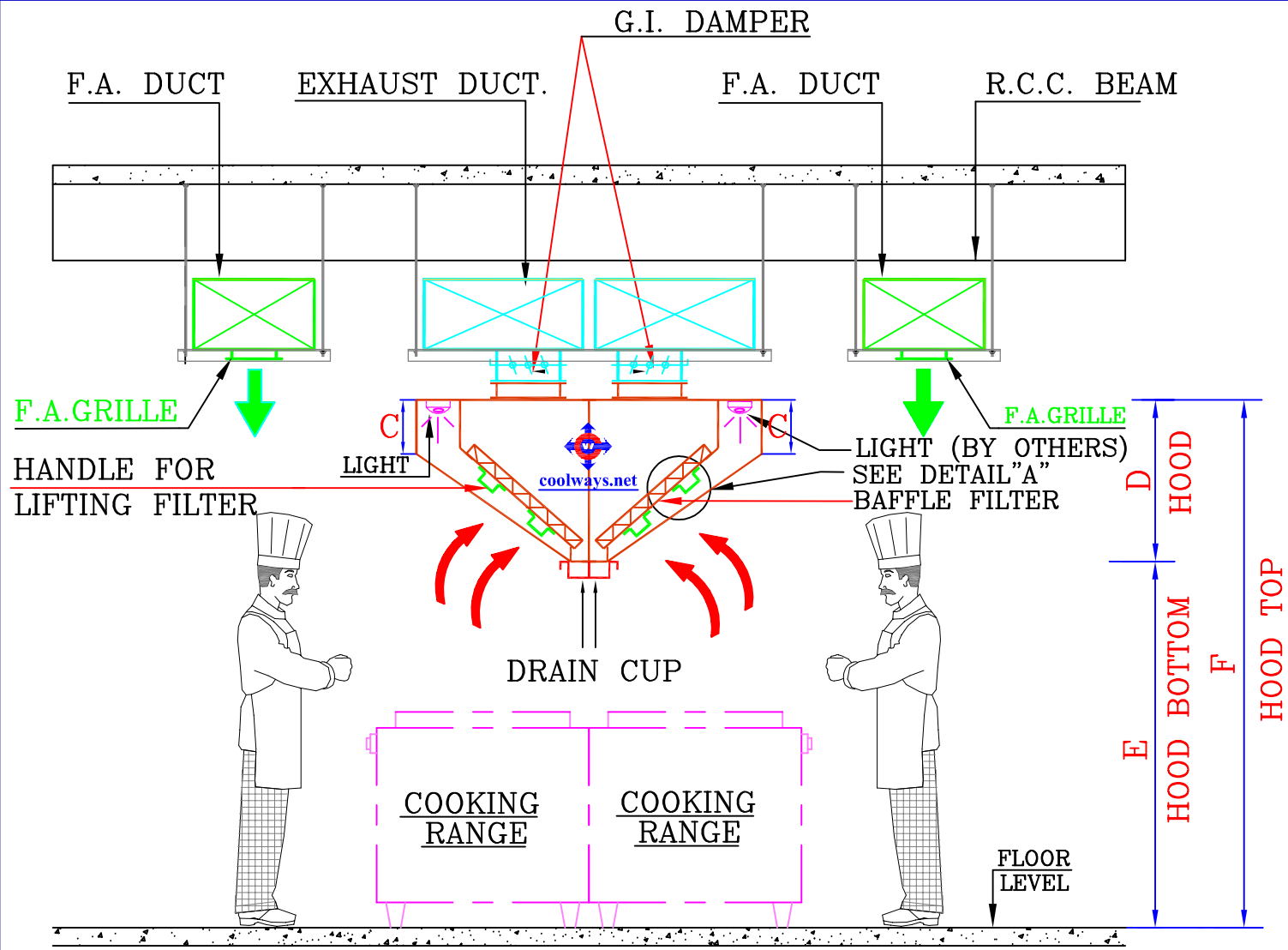
ISLAND TYPE CEILING SUSPENDED HOOD SECTION VIEW.
