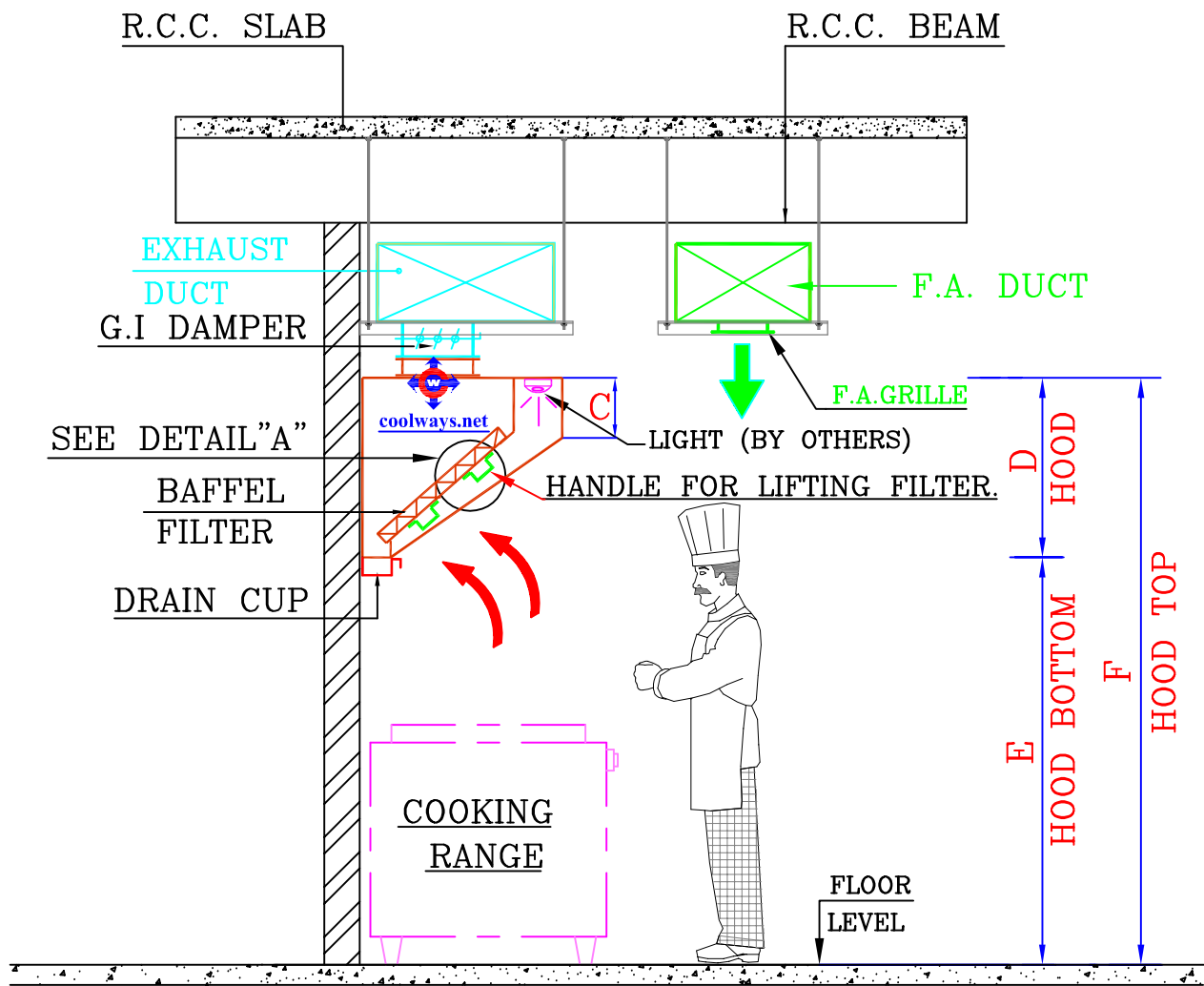
WALL MOUNTED. HOOD SECTION VIEW.
