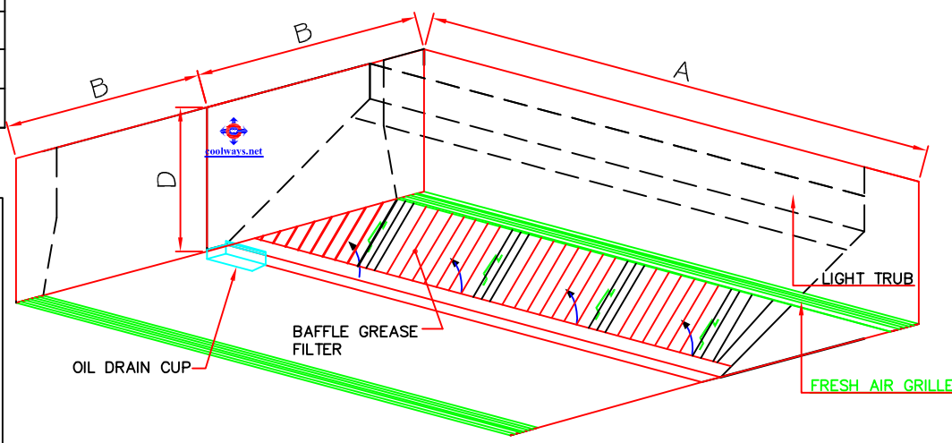
ISOMETRIC VIEW CANOPY TYPE (ISLAND MOUNTED).
