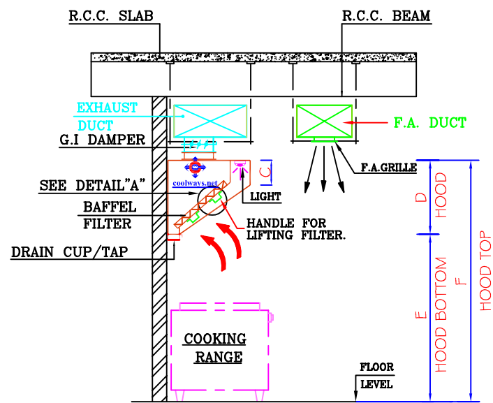
WALL MOUNTED. HOOD SECTION VIEW.
