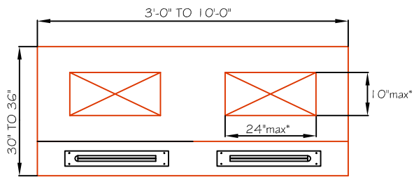
WALL MOUNTED. HOOD PLAN VIEW.
