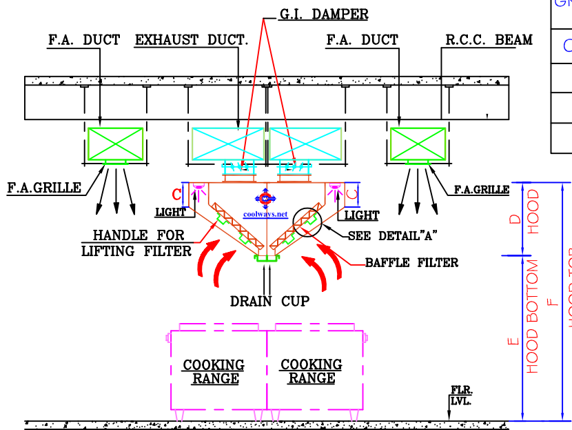
ISLAND MOUNTED. HOOD SECTION VIEW.
