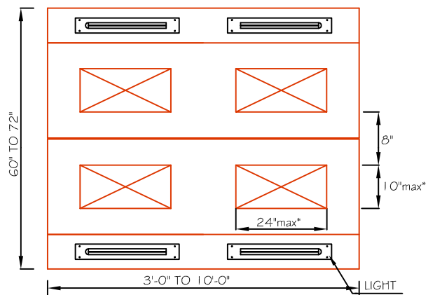
ISLAND MOUNTED. HOOD PLAN VIEW.
