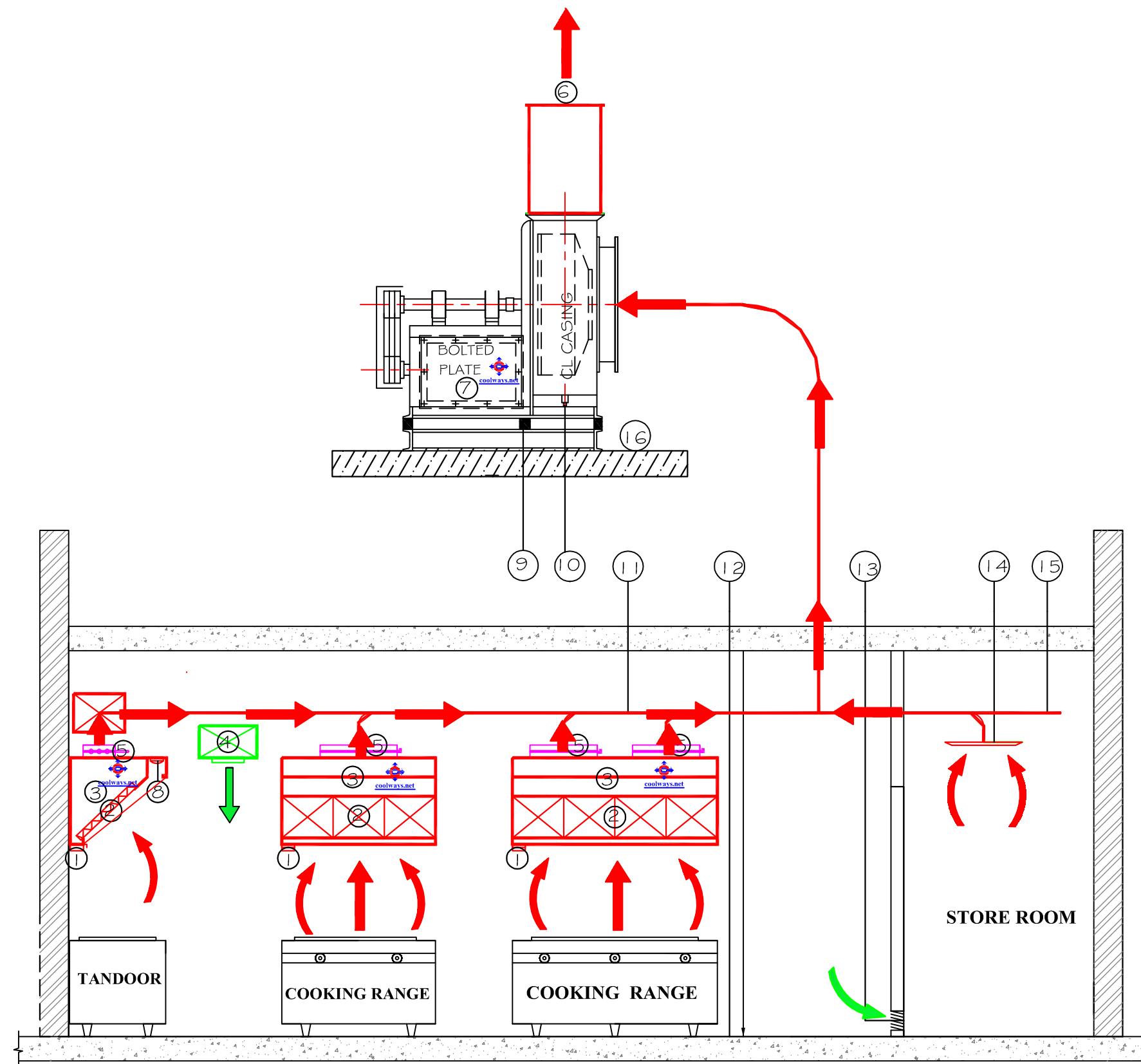
KITCHEN EXHAUST SYSTEM SCHEMATIC DIAGRAM
